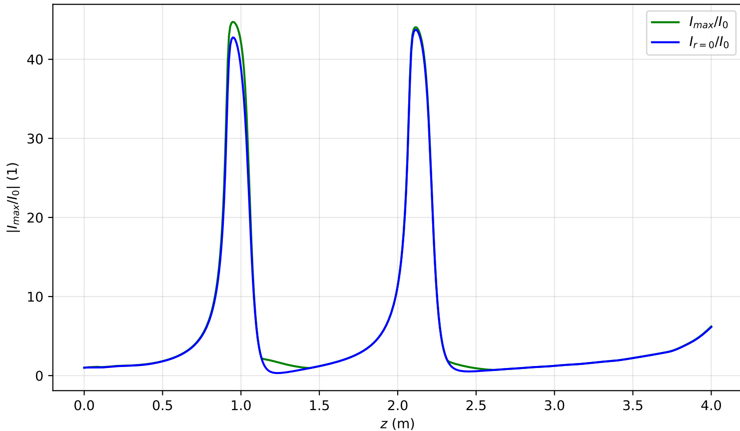
I_{max}(x=0, y=0, z)/I_0 , Pin=2.4Pcr, noisy input, artificial time
